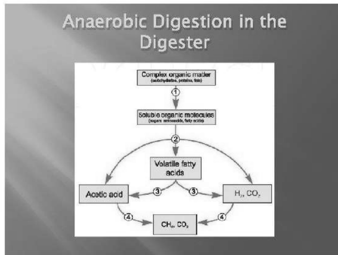
The key process stages of anaerobic digestion
